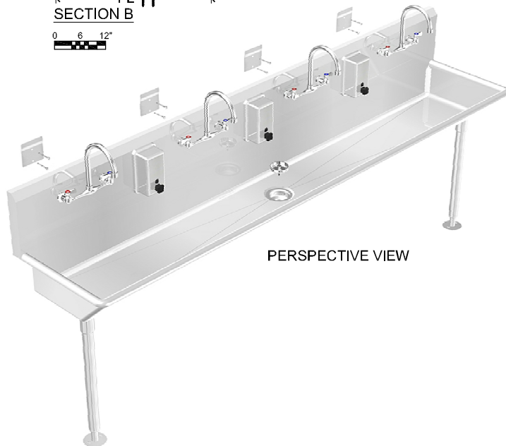
FAUCET PERSPECTIVE VIEW MODEL: BSMAA-700
